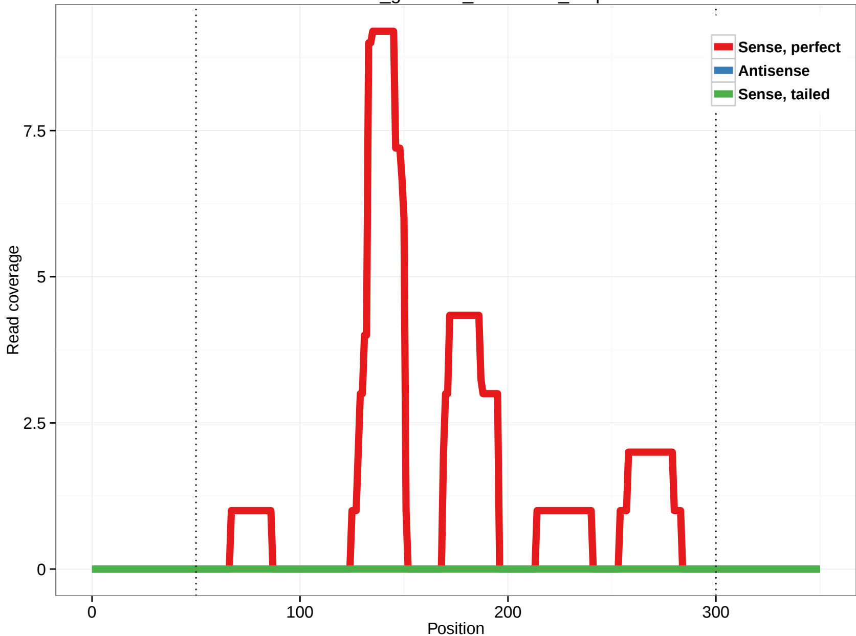
rheMac3_genscan_chr1.3006_1.5p
