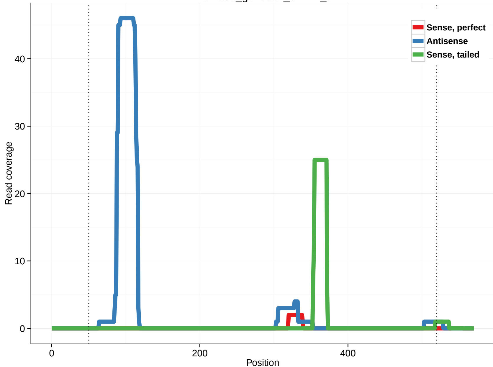
rheMac3_genscan_chr1.2_9
