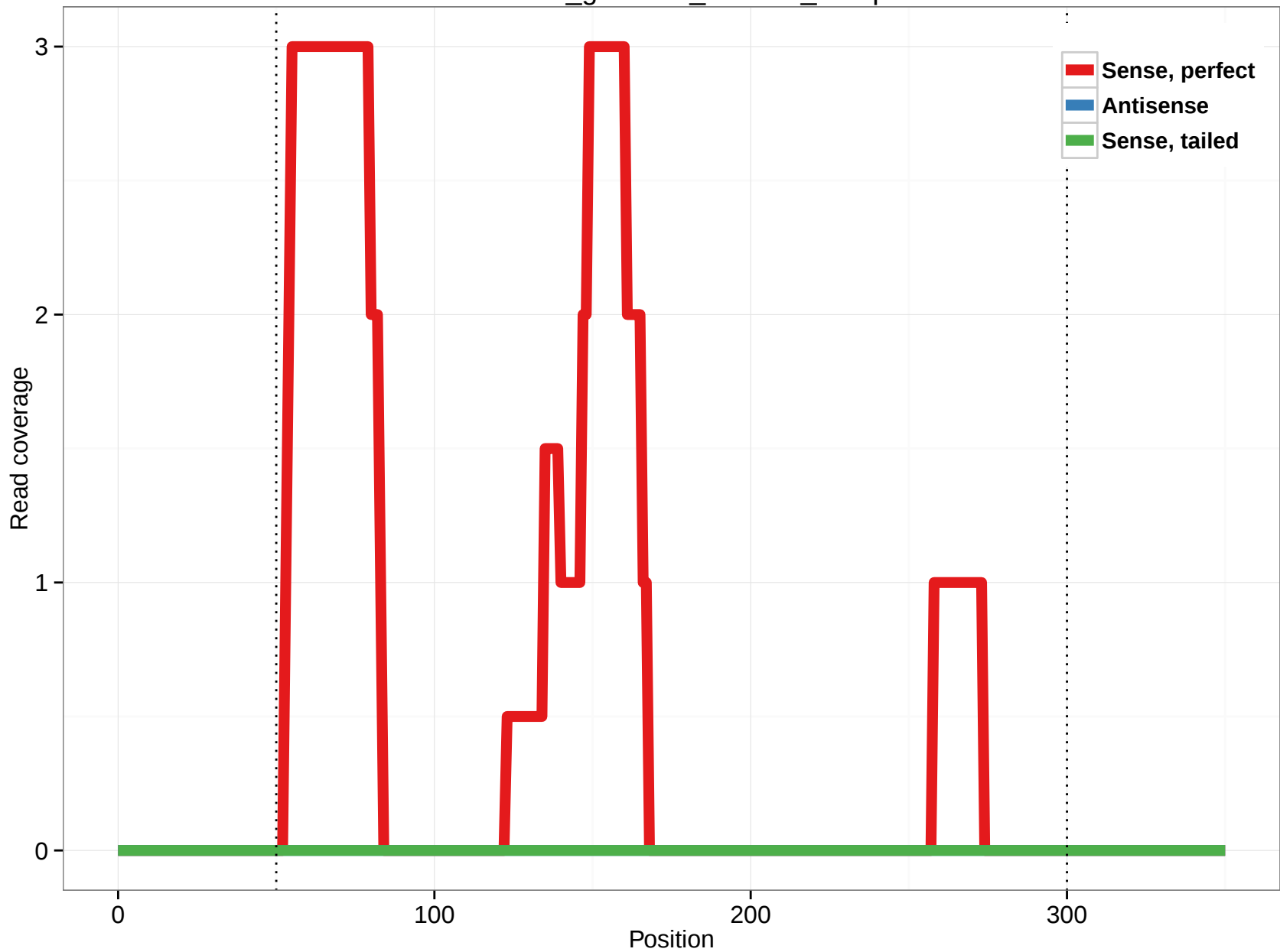
rheMac3_genscan_chr1.29_10.3p
