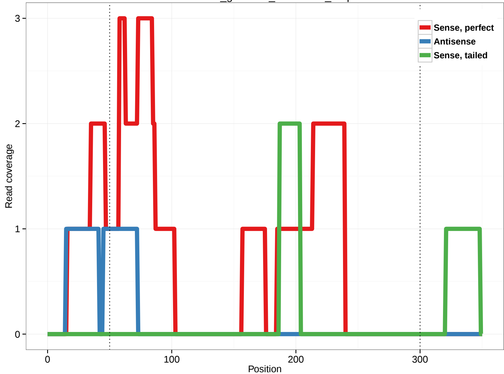
rheMac3_genscan_chr1.2987_9.3p
