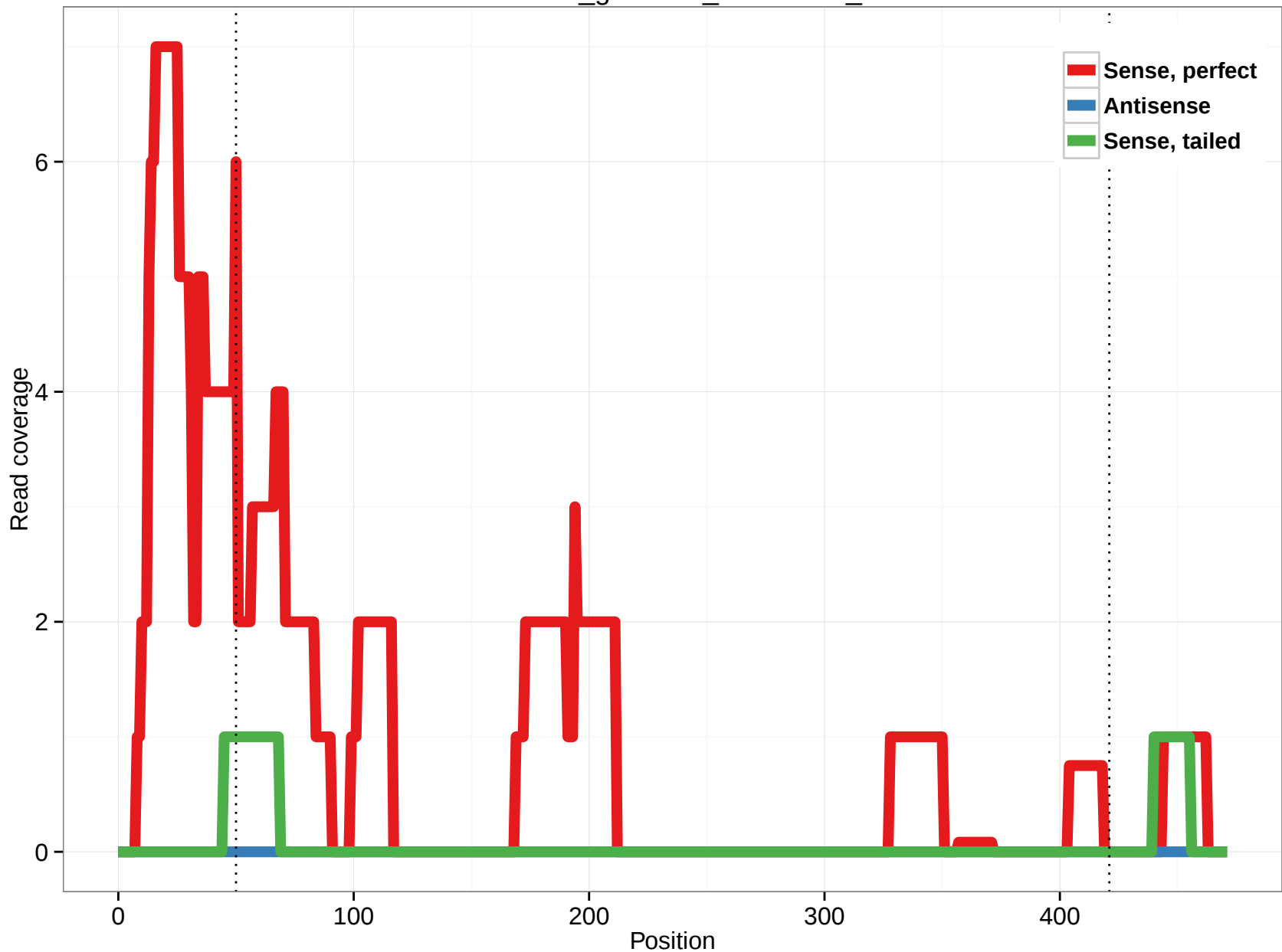
rheMac3_genscan_chr1.2941_1
