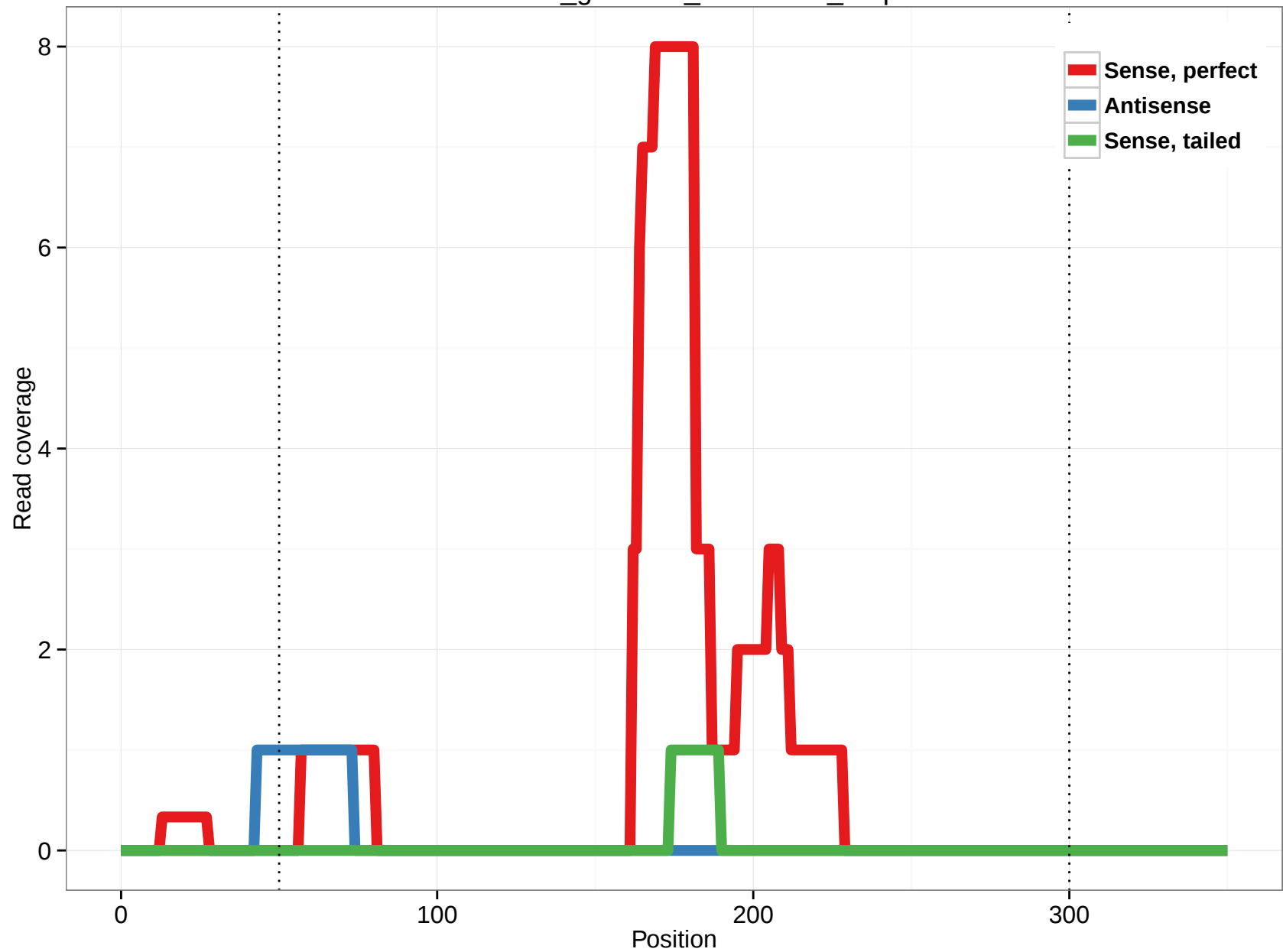
rheMac3_genscan_chr1.2940_0.5p
