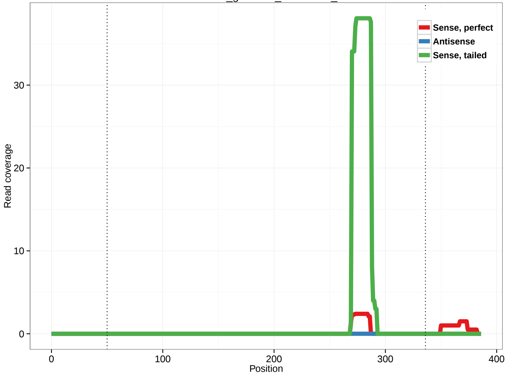
rheMac3_genscan_chr1.2908_27
