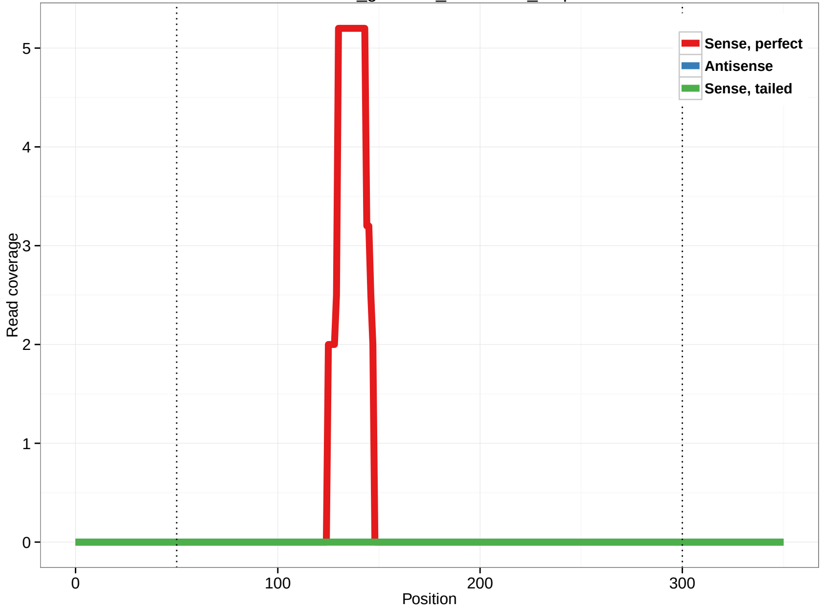
rheMac3_genscan_chr1.2907_7.5p
