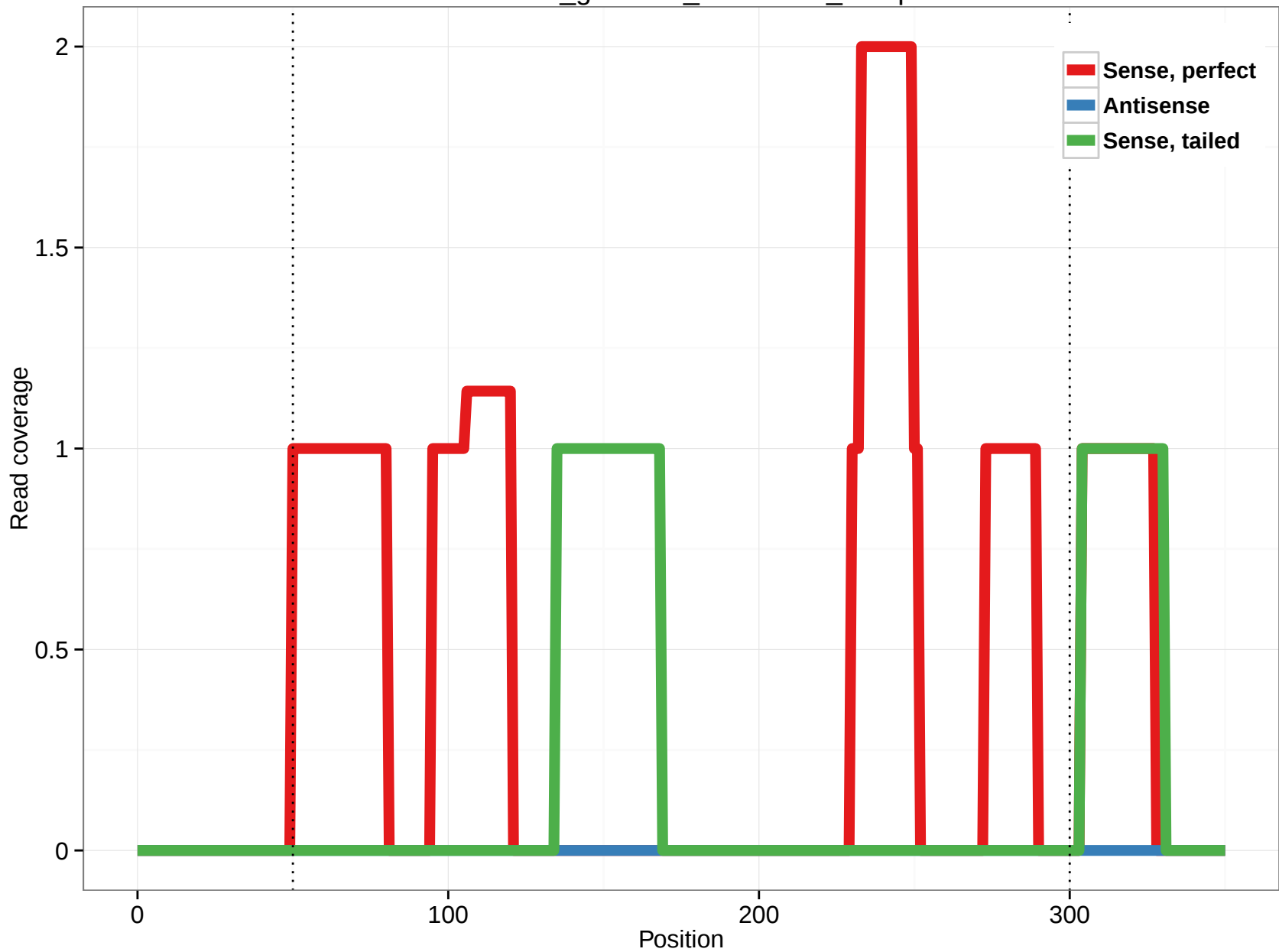
rheMac3_genscan_chr1.2905_25.5p
