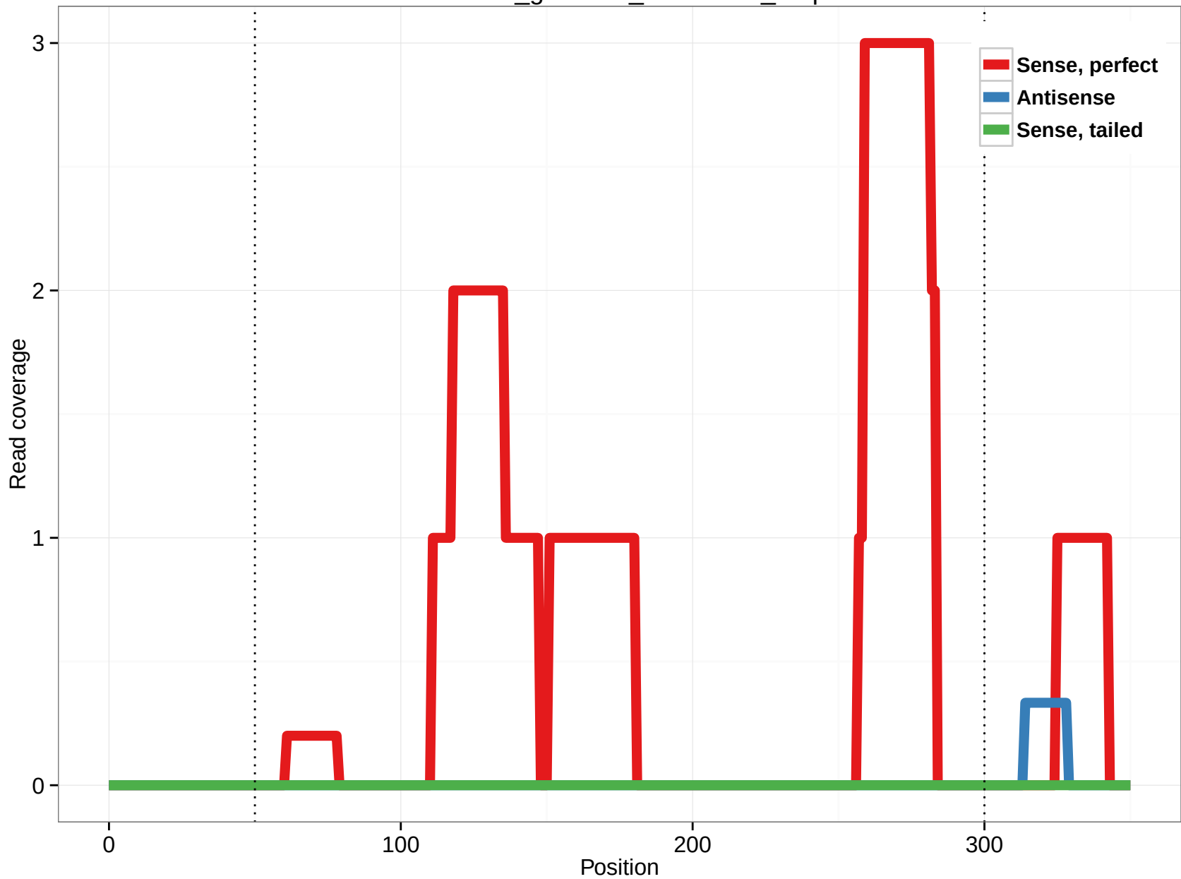
rheMac3_genscan_chr1.2903_3.5p
