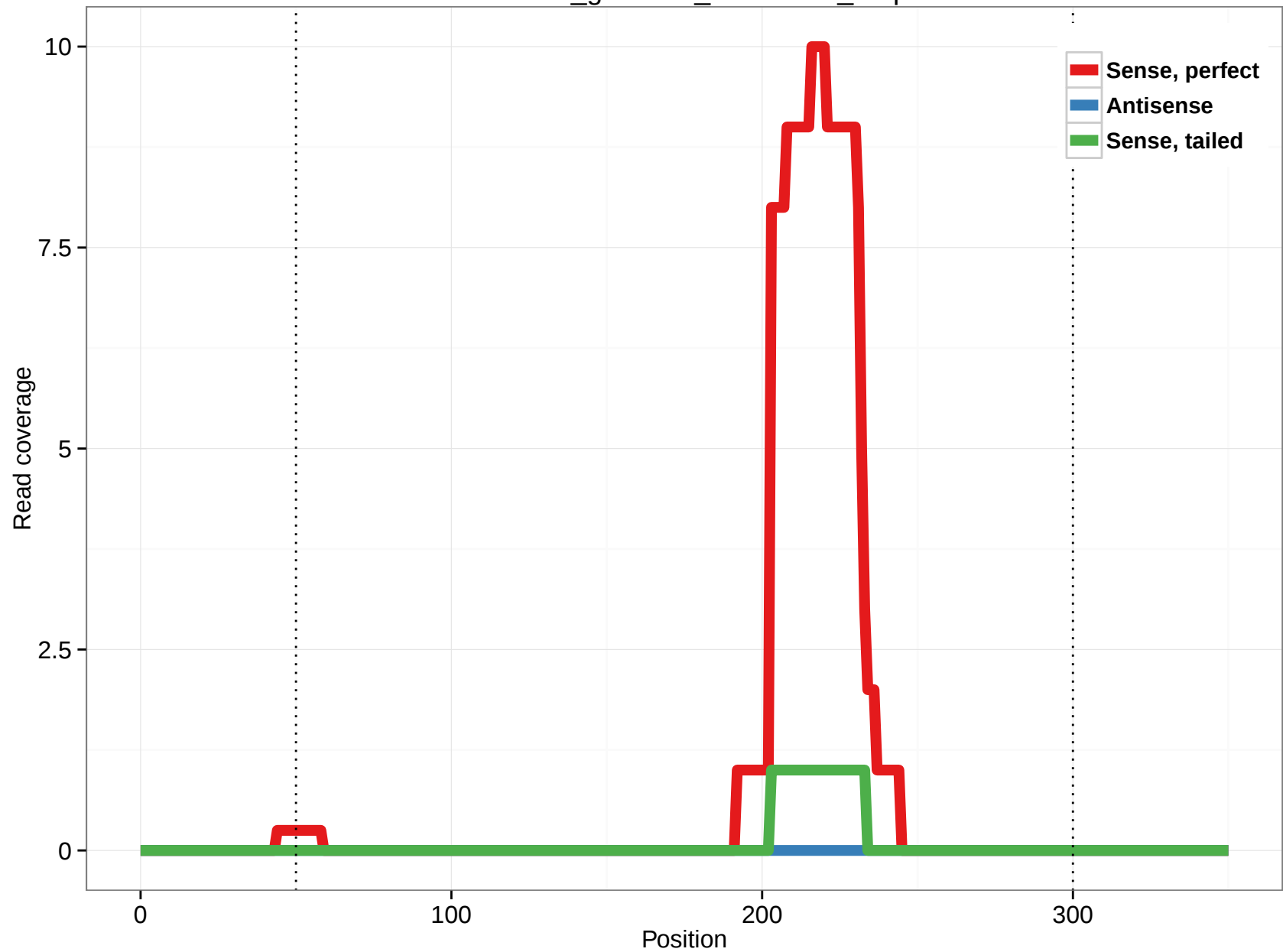
rheMac3_genscan_chr1.2903_2.3p
