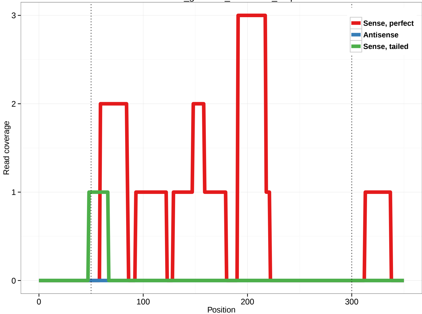
rheMac3_genscan_chr1.2900_5.5p
