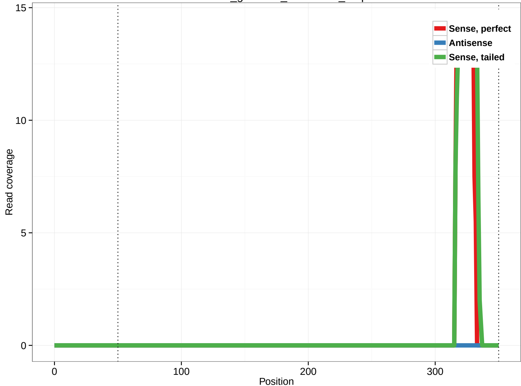
rheMac3_genscan_chr1.2836_0.5p
