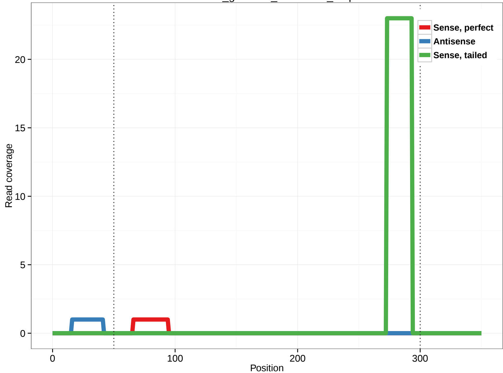
rheMac3_genscan_chr1.2834_7.5p
