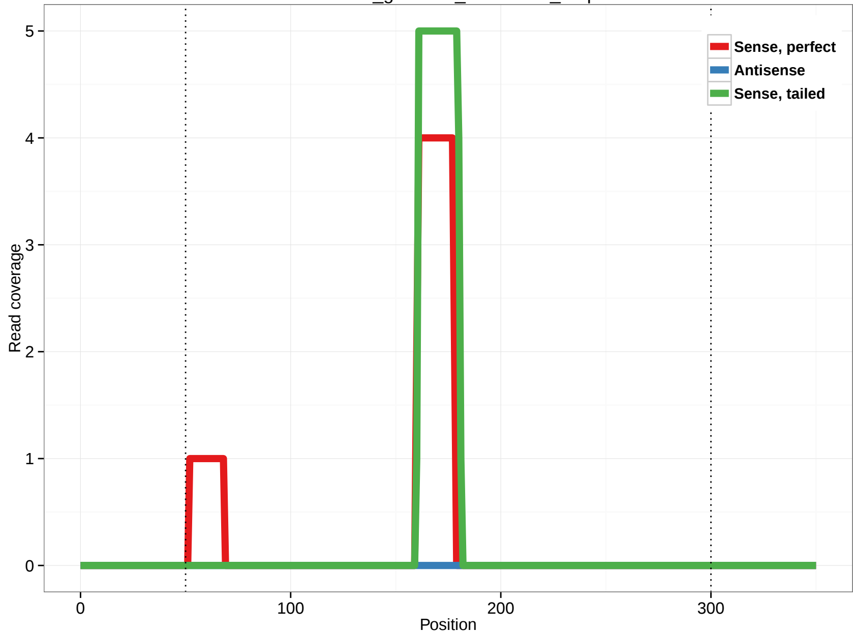
rheMac3_genscan_chr1.2814_6.5p
