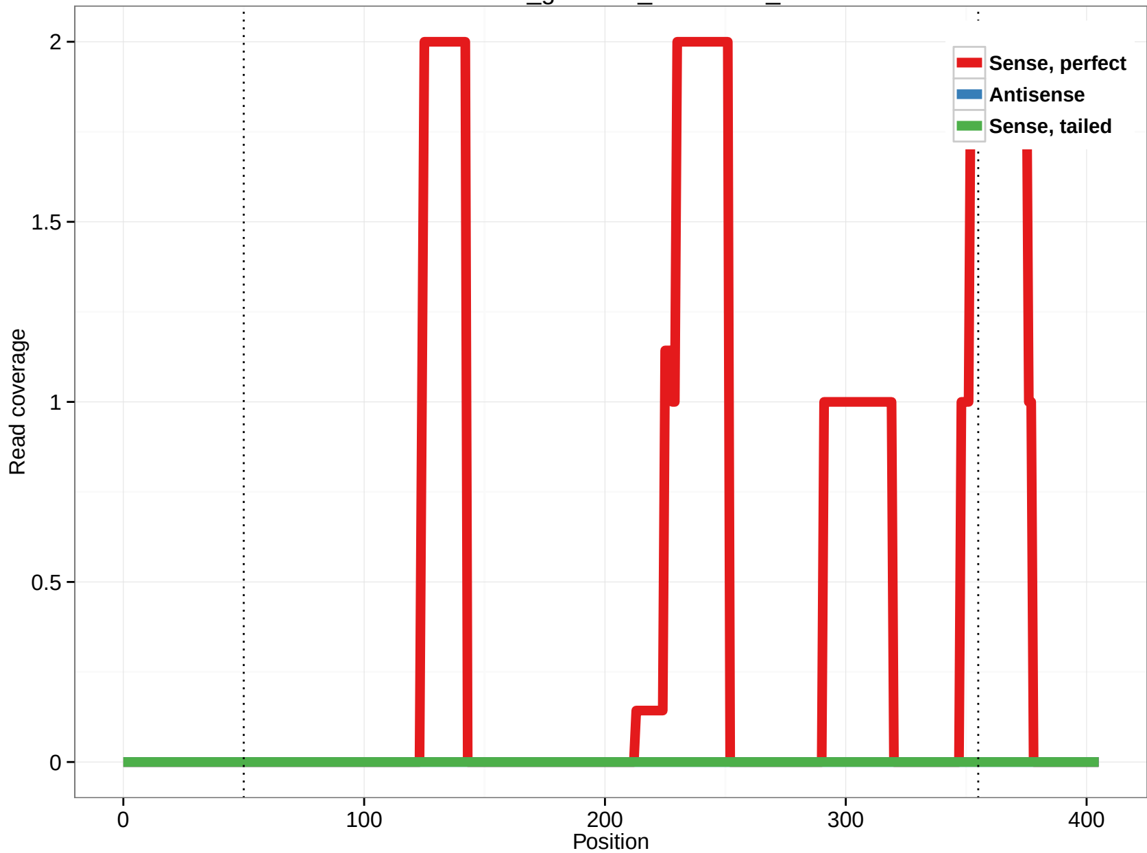
rheMac3_genscan_chr1.2789_0
