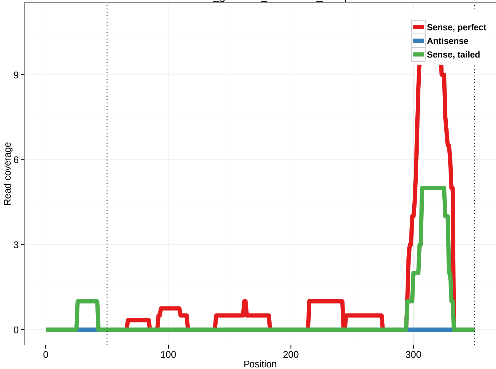
rheMac3_genscan_chr1.2788_11.5p
