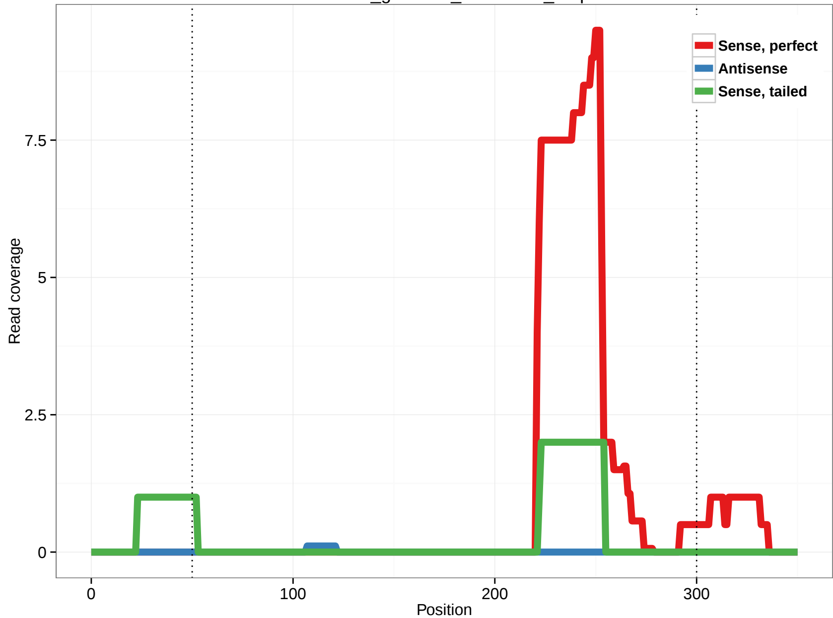
rheMac3_genscan_chr1.2767_5.5p
