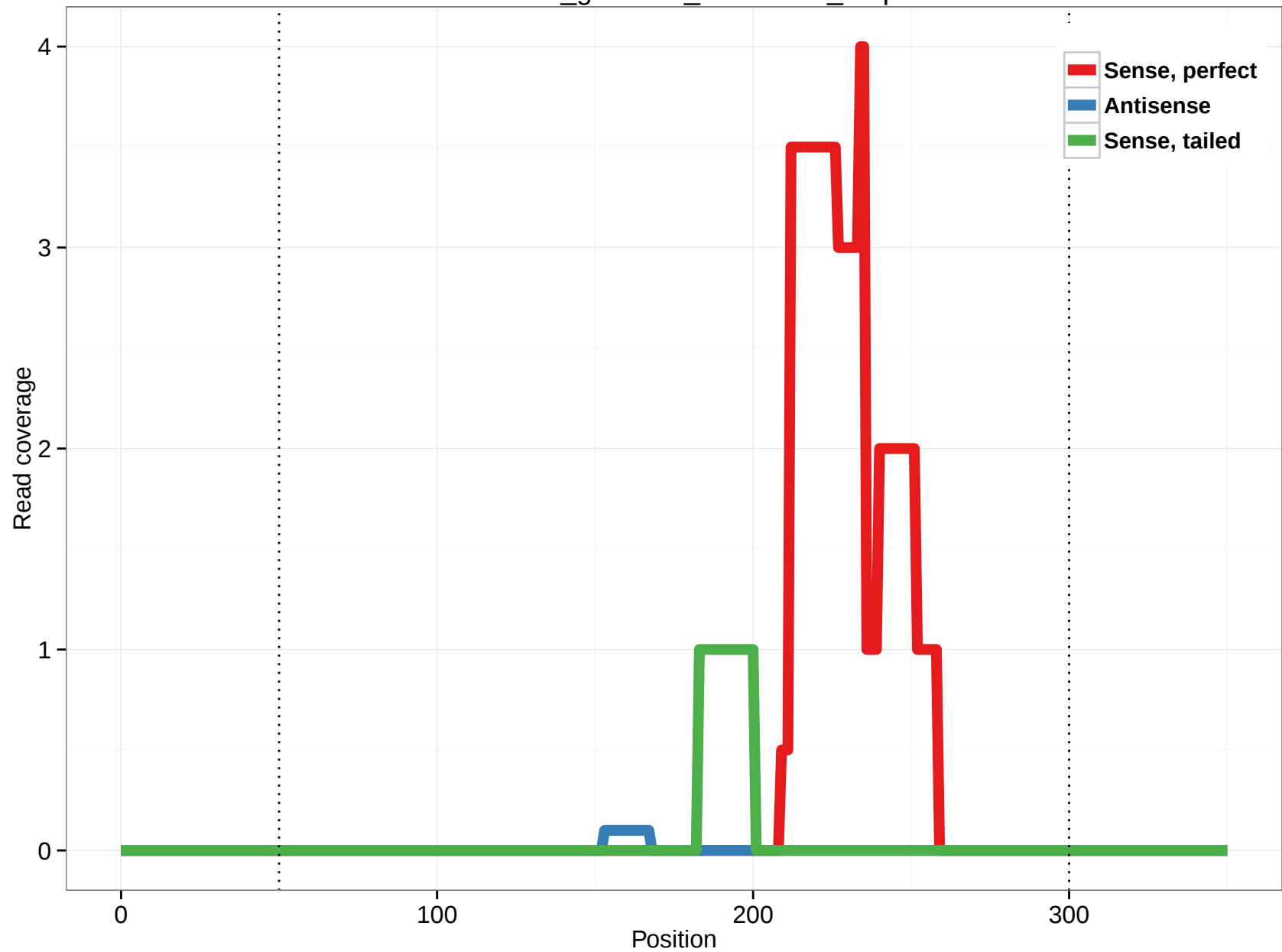
rheMac3_genscan_chr1.2764_0.3p
