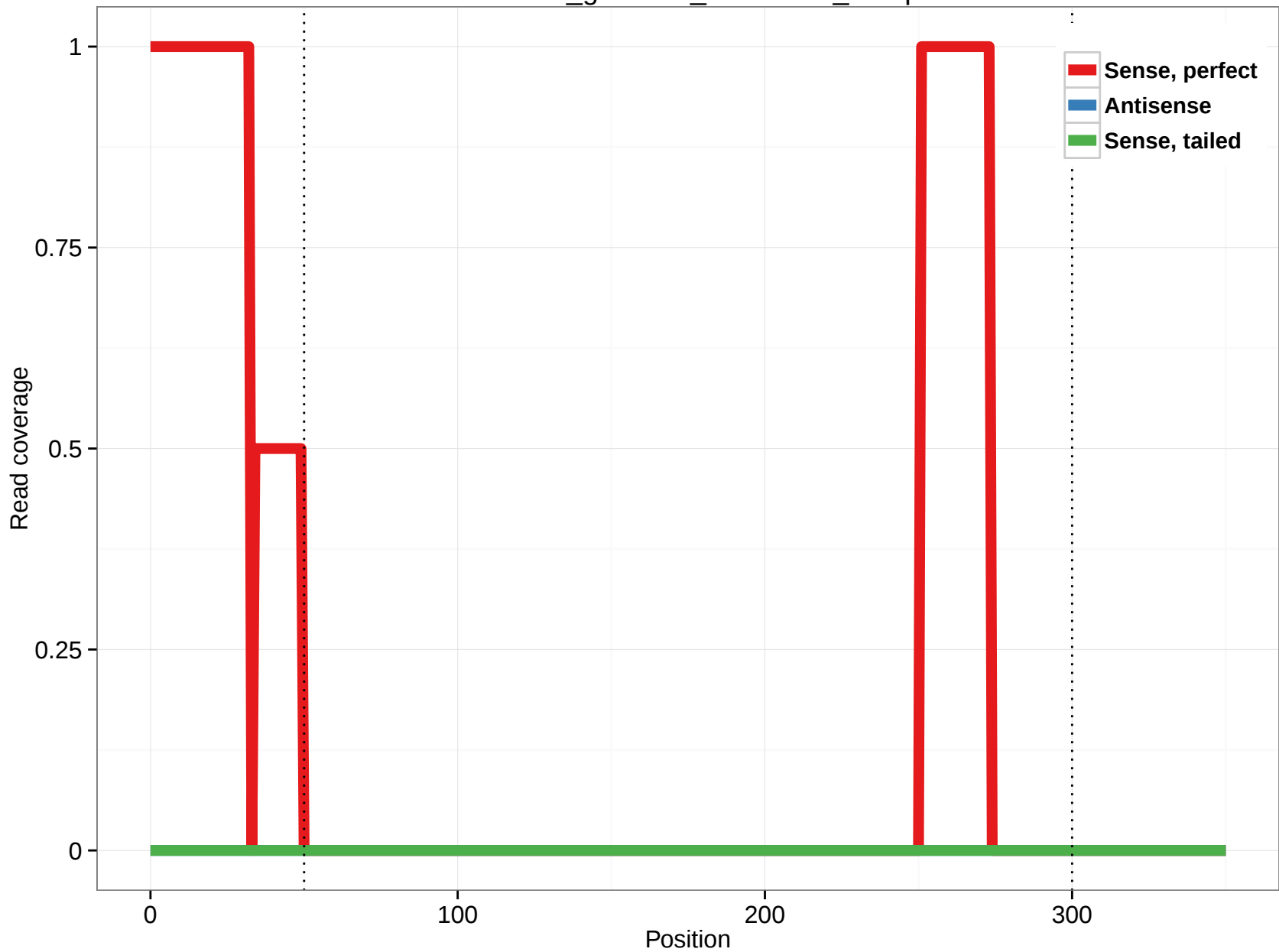
rheMac3_genscan_chr1.2763_16.5p
