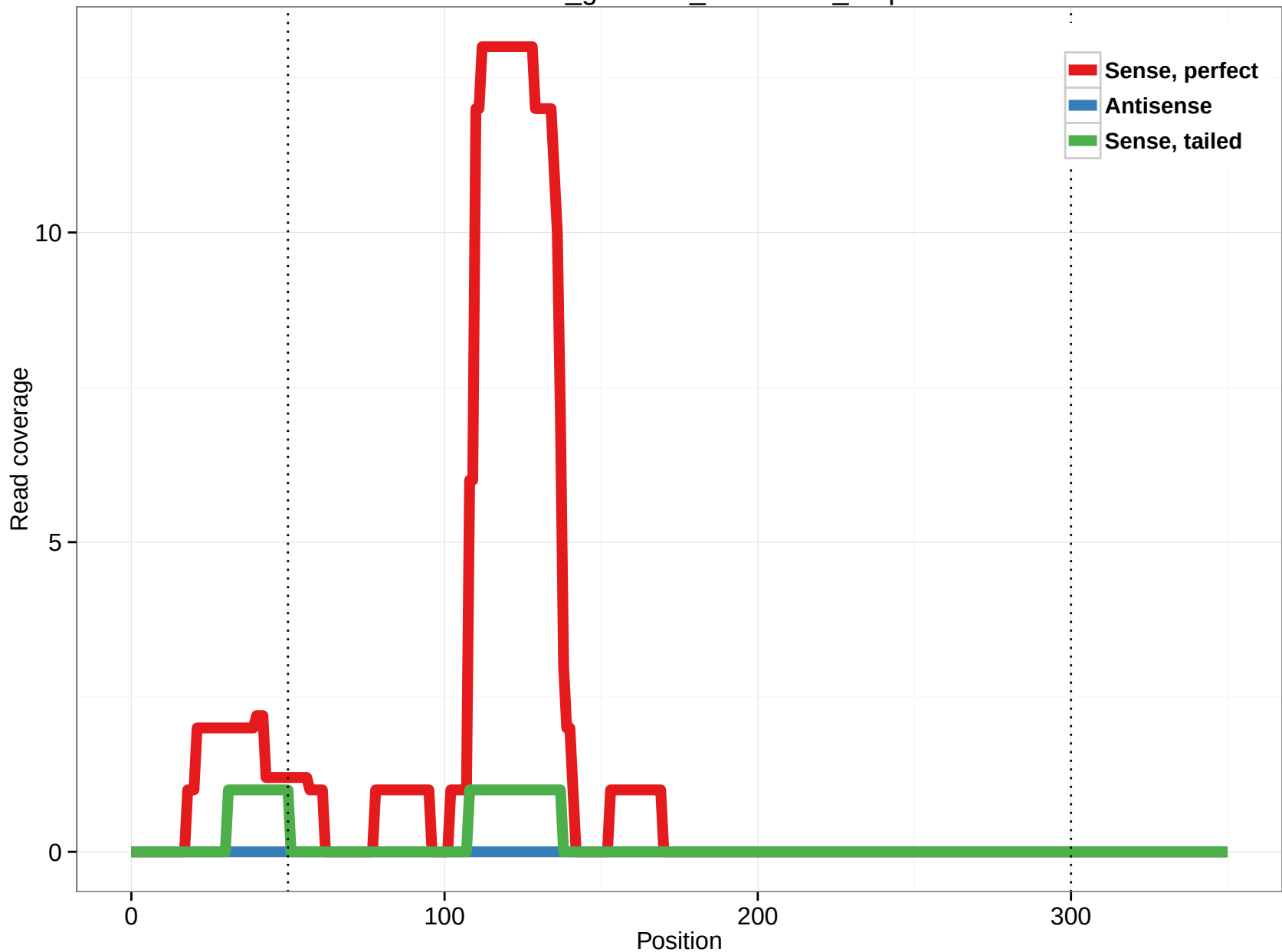
rheMac3_genscan_chr1.2762_1.5p
