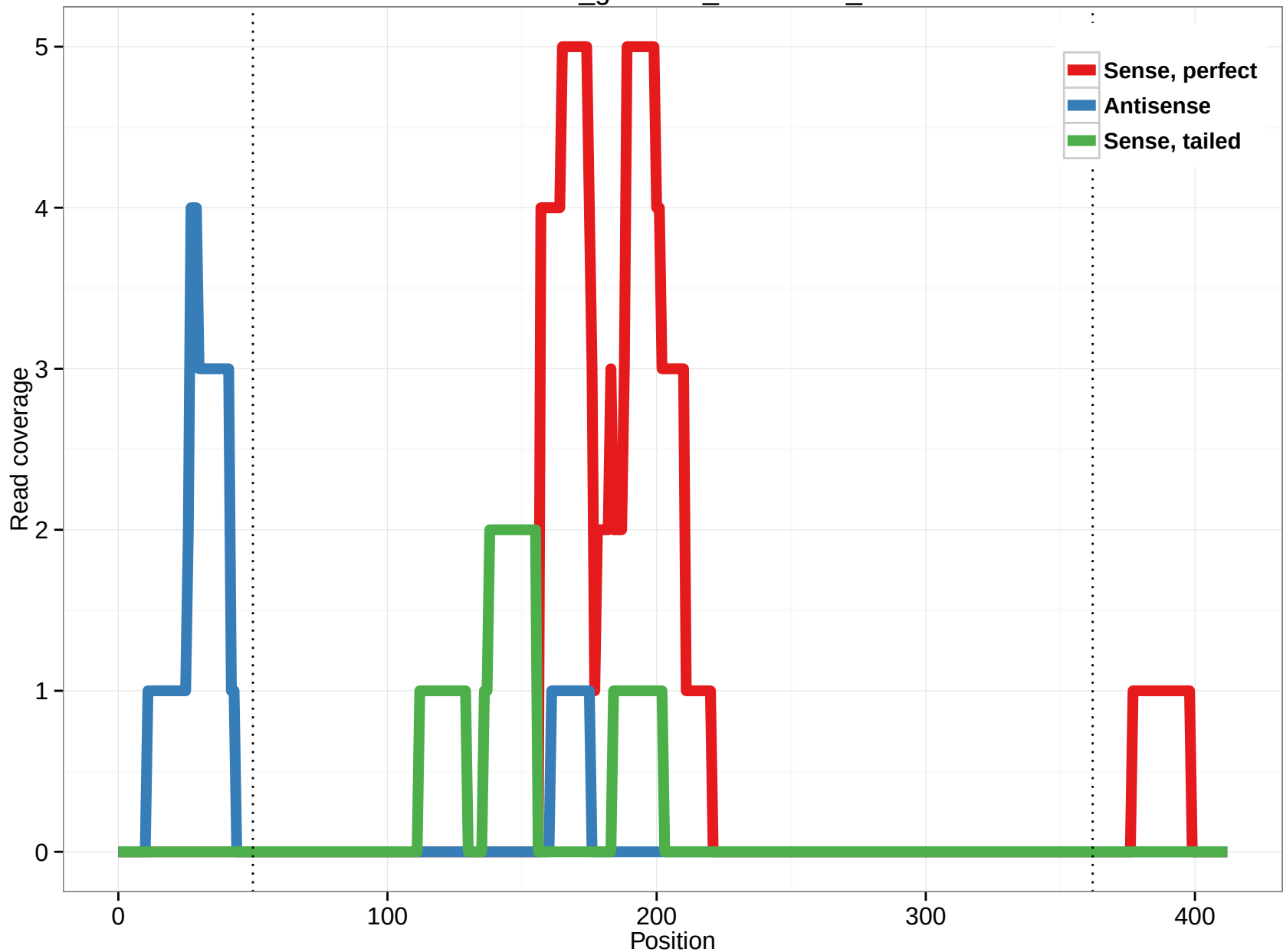
rheMac3_genscan_chr1.2759_0
