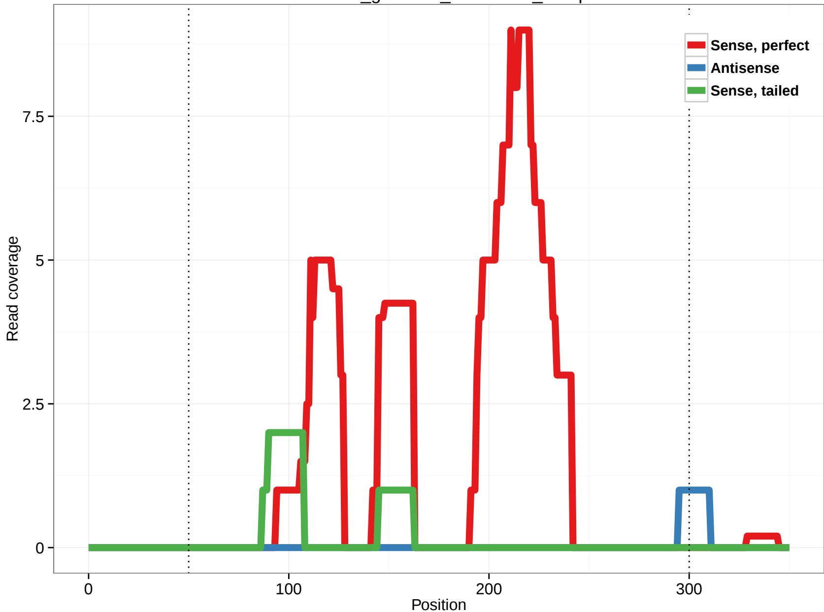
rheMac3_genscan_chr1.2743_29.3p
