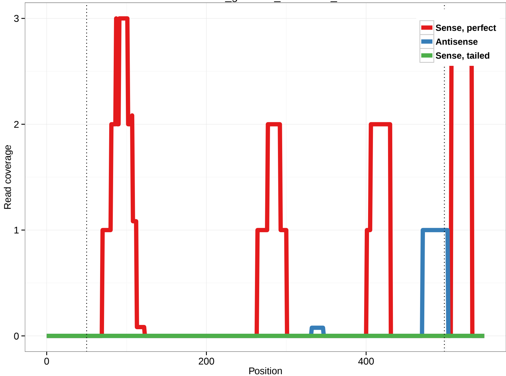
rheMac3_genscan_chr1.2743_11
