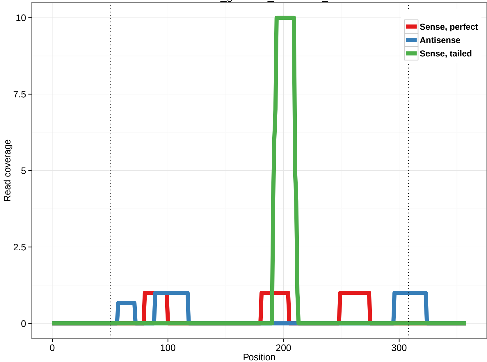
rheMac3_genscan_chr1.2734_26
