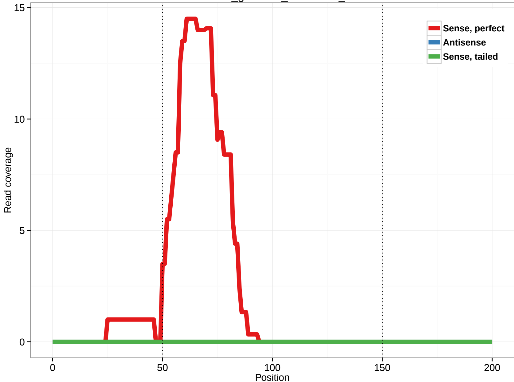
rheMac3_genscan_chr1.2734_11
