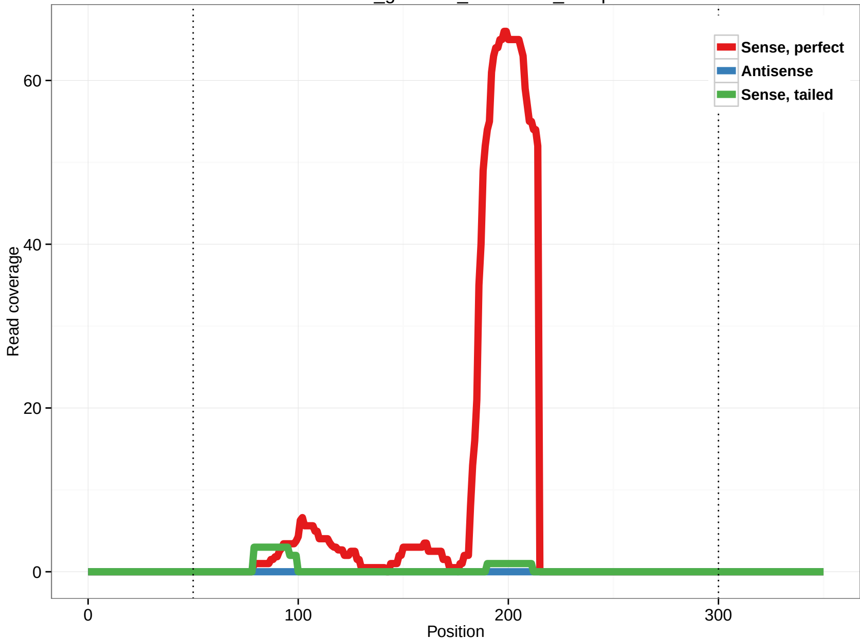
rheMac3_genscan_chr1.2732_17.3p
