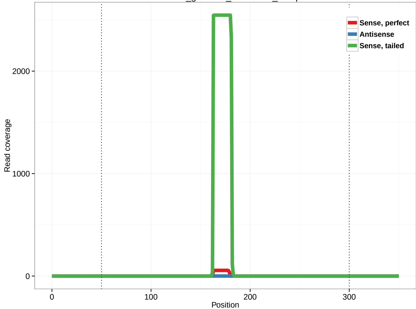
rheMac3_genscan_chr1.2709_11.5p
