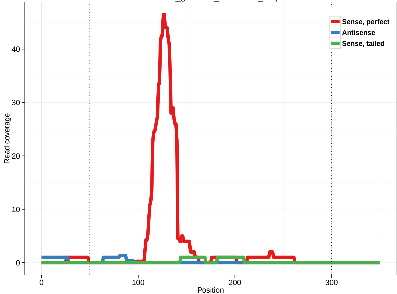
rheMac3_genscan_chr1.2699_0.3p
