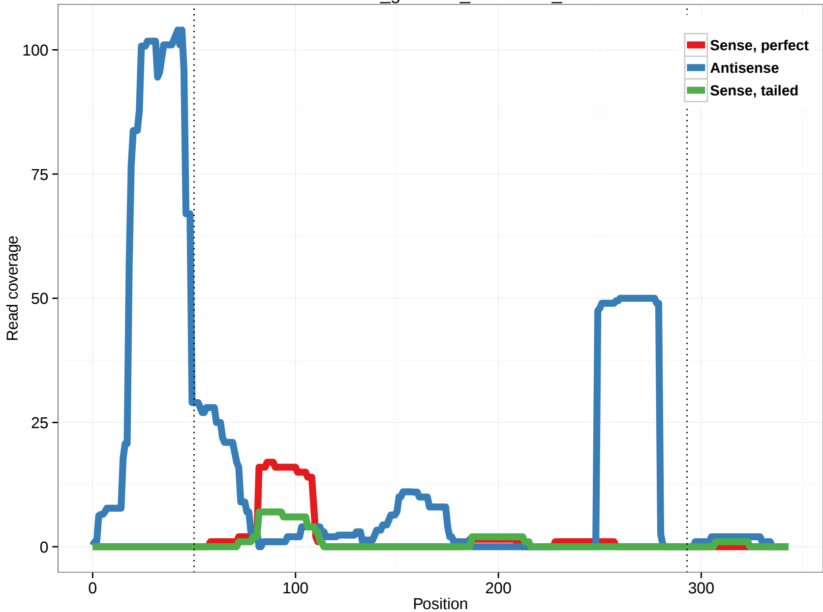
rheMac3_genscan_chr1.2648_5
