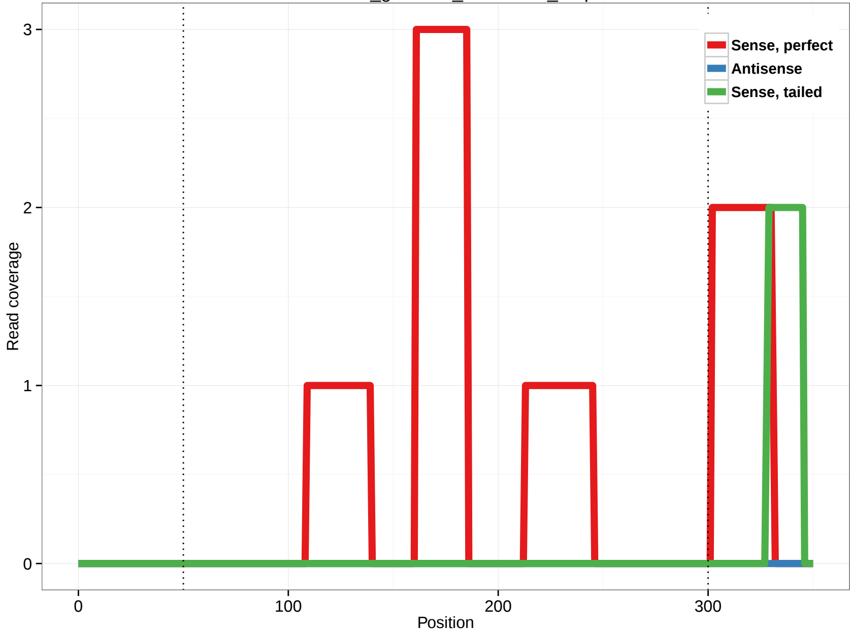
rheMac3_genscan_chr1.2637_2.3p
