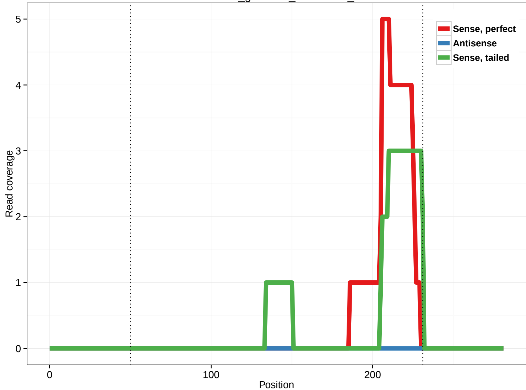
rheMac3_genscan_chr1.2635_0
