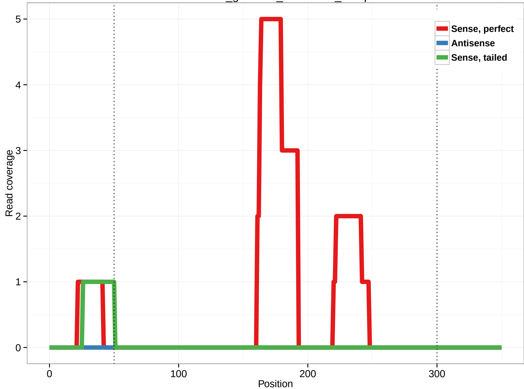
rheMac3_genscan_chr1.2633_41.5p
