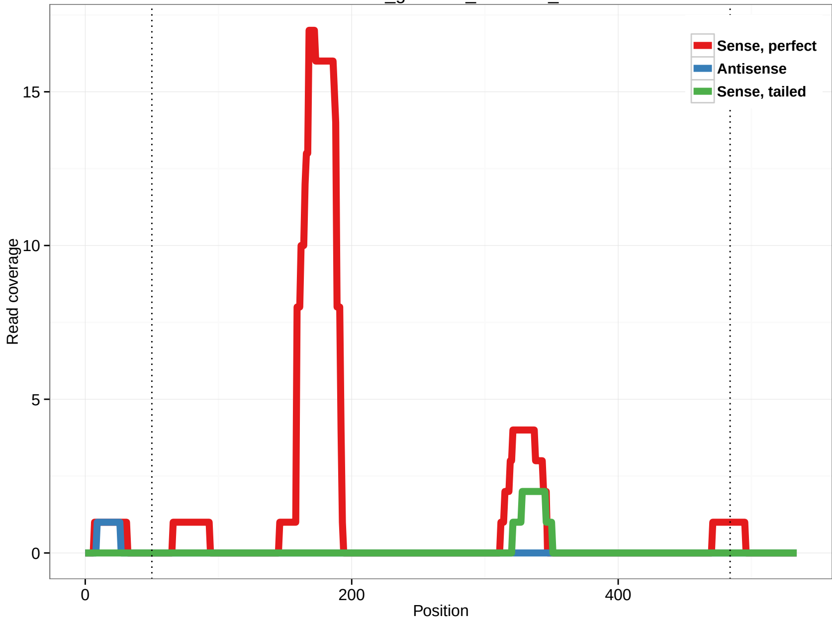
rheMac3_genscan_chr1.262_1
