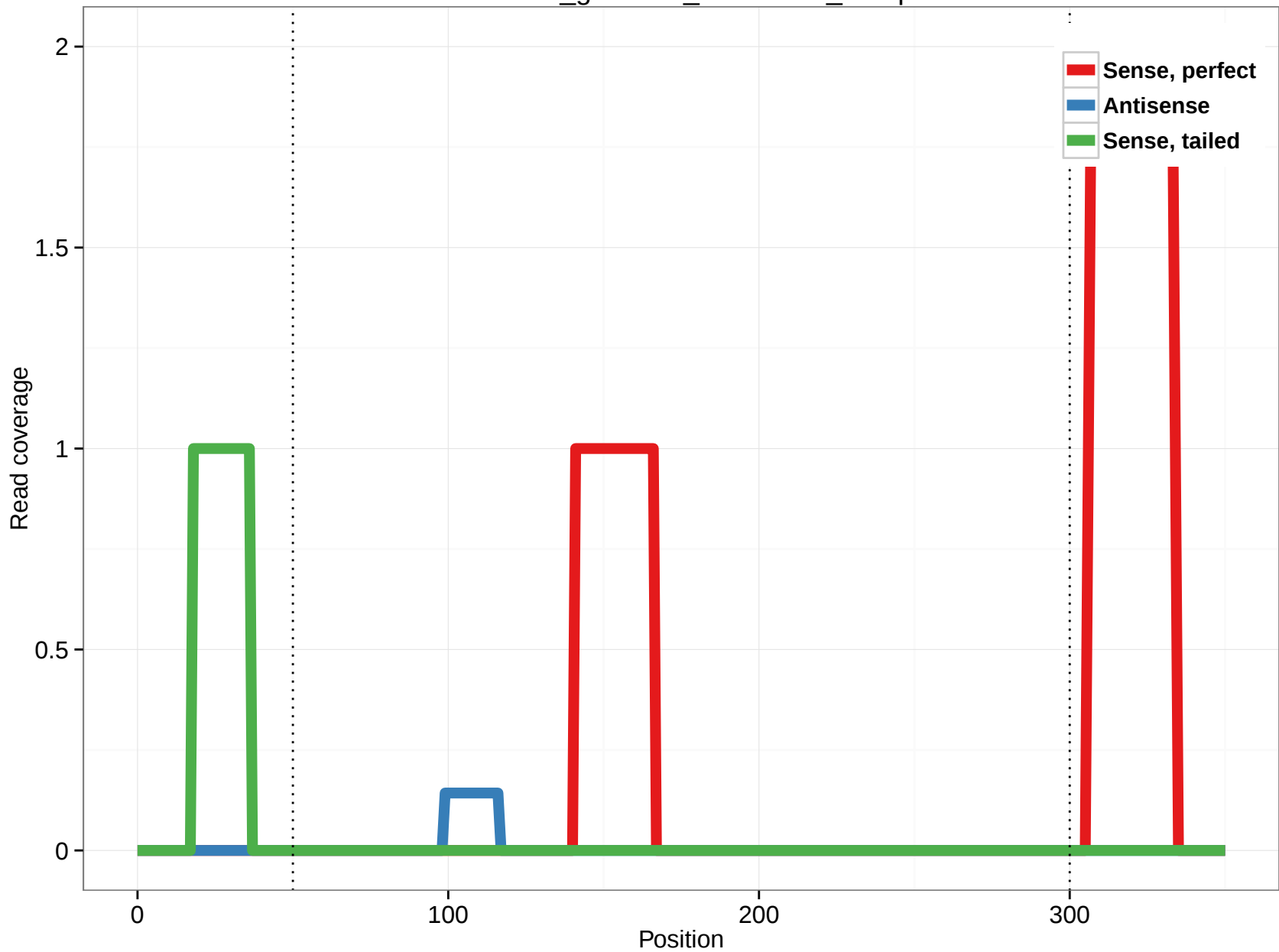
rheMac3_genscan_chr1.2629_15.3p
