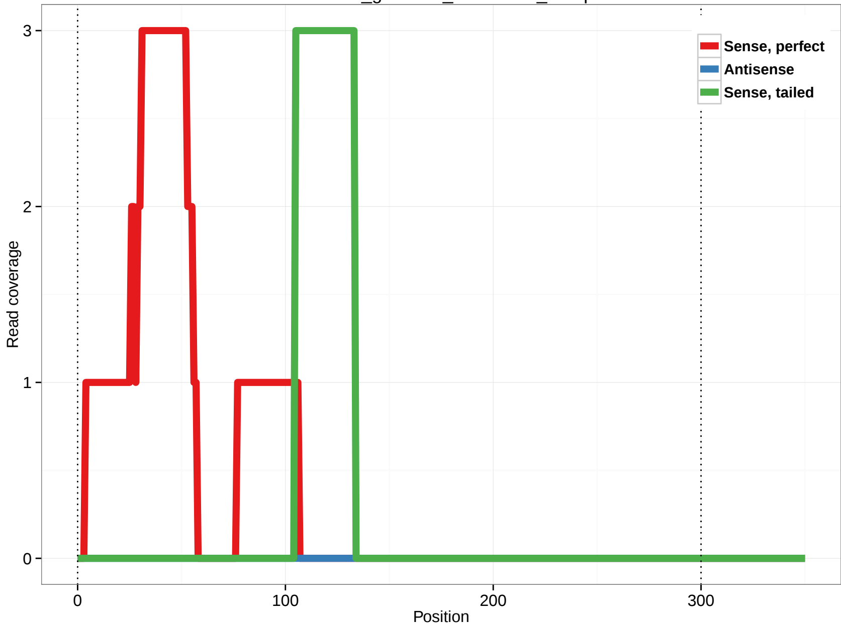
rheMac3_genscan_chr1.2627_11.3p
