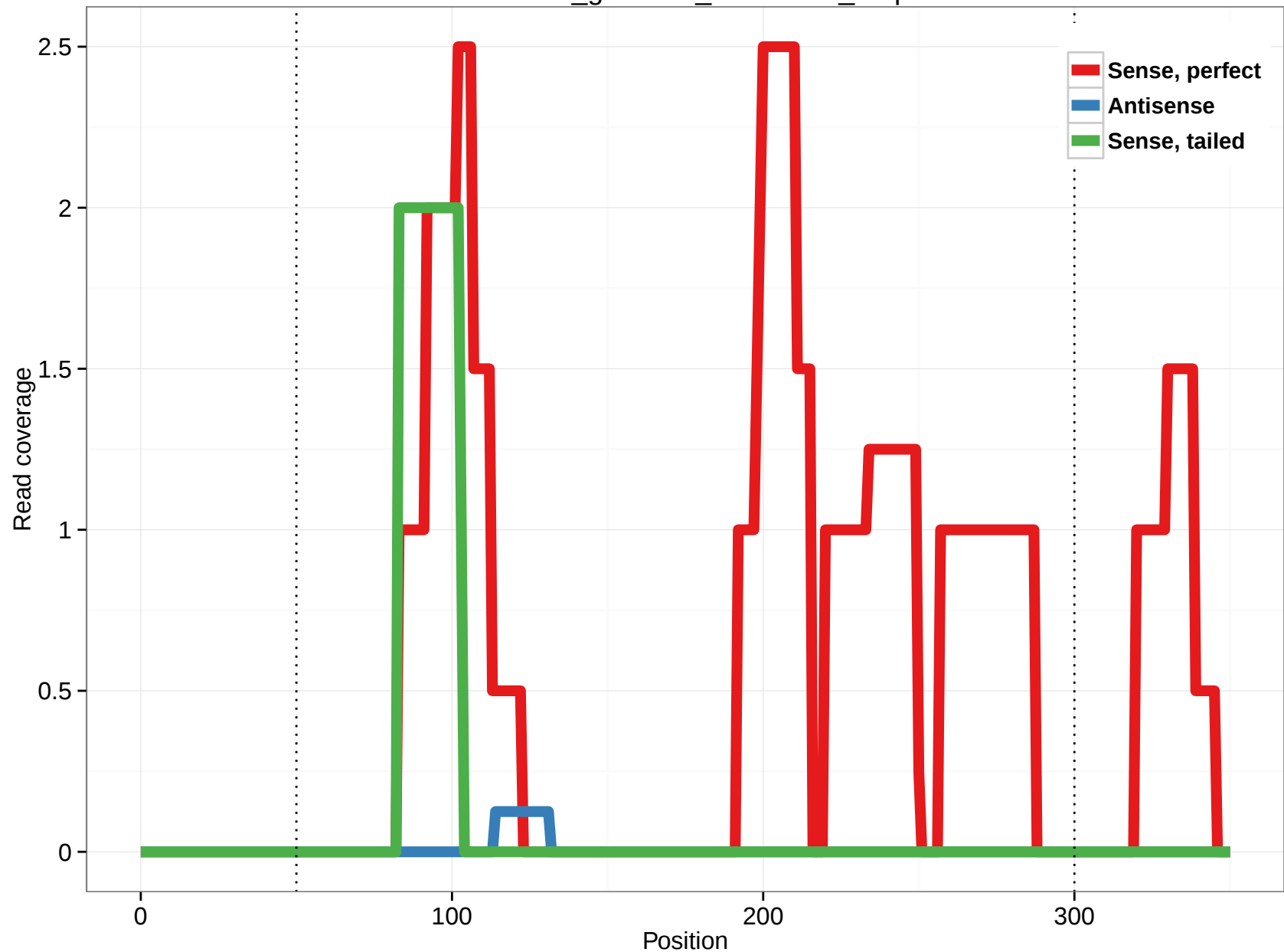
rheMac3_genscan_chr1.2570_0.5p
