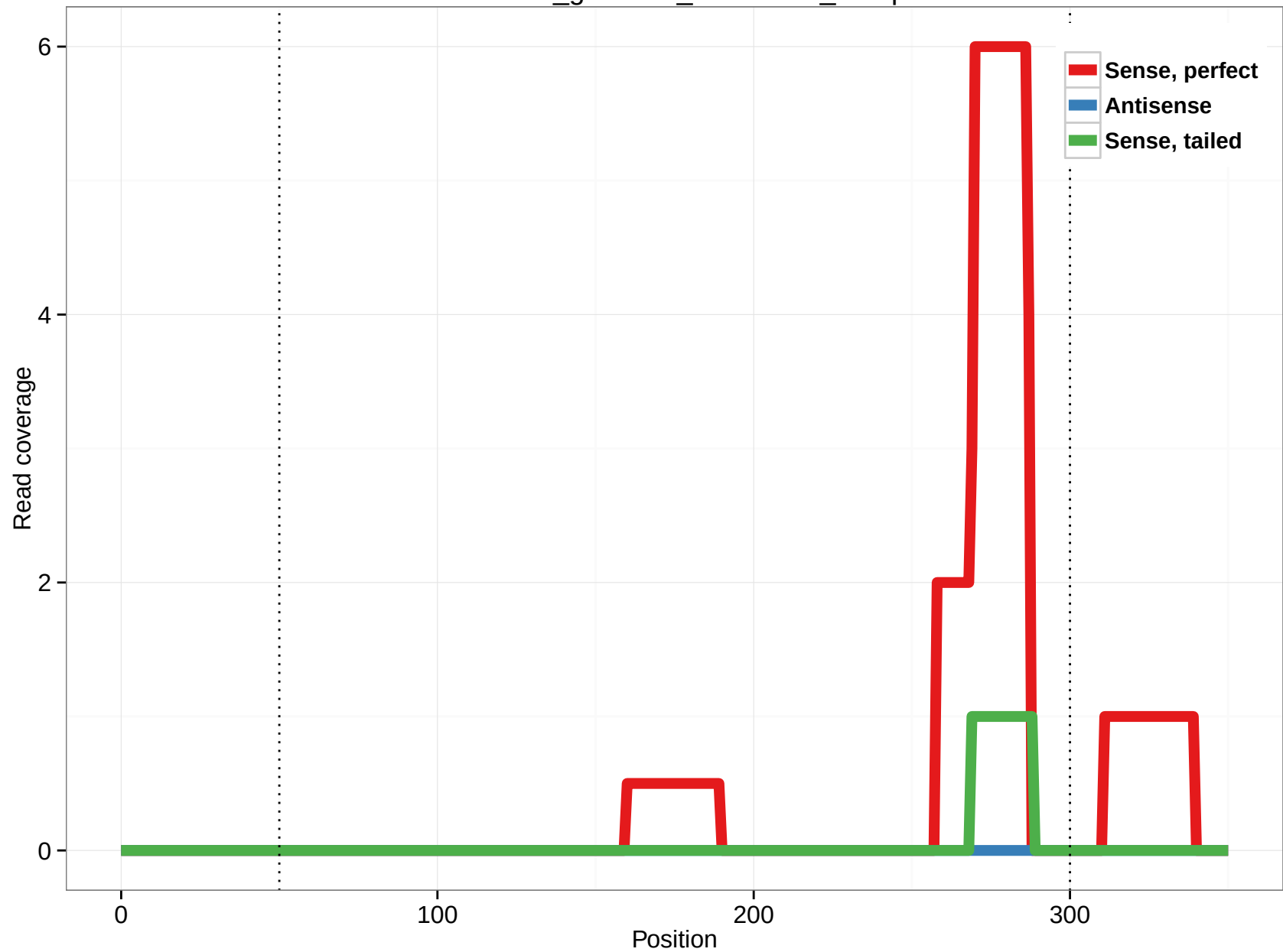
rheMac3_genscan_chr1.2542_11.5p
