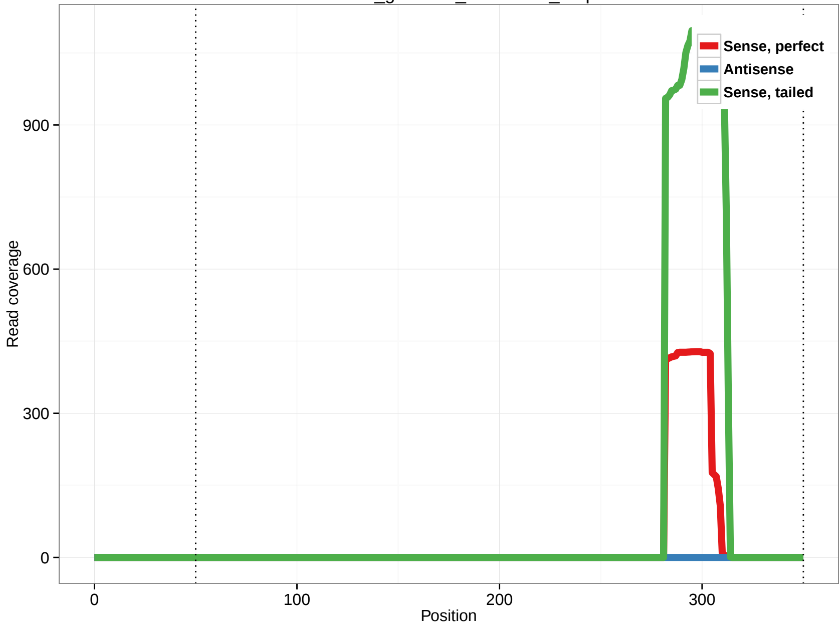
rheMac3_genscan_chr1.2538_2.5p
