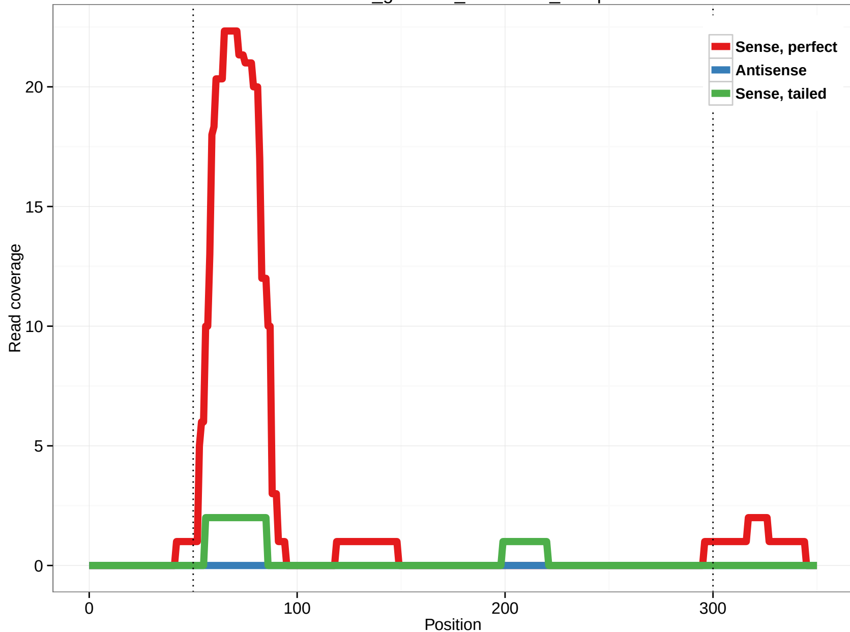
rheMac3_genscan_chr1.2526_12.3p
