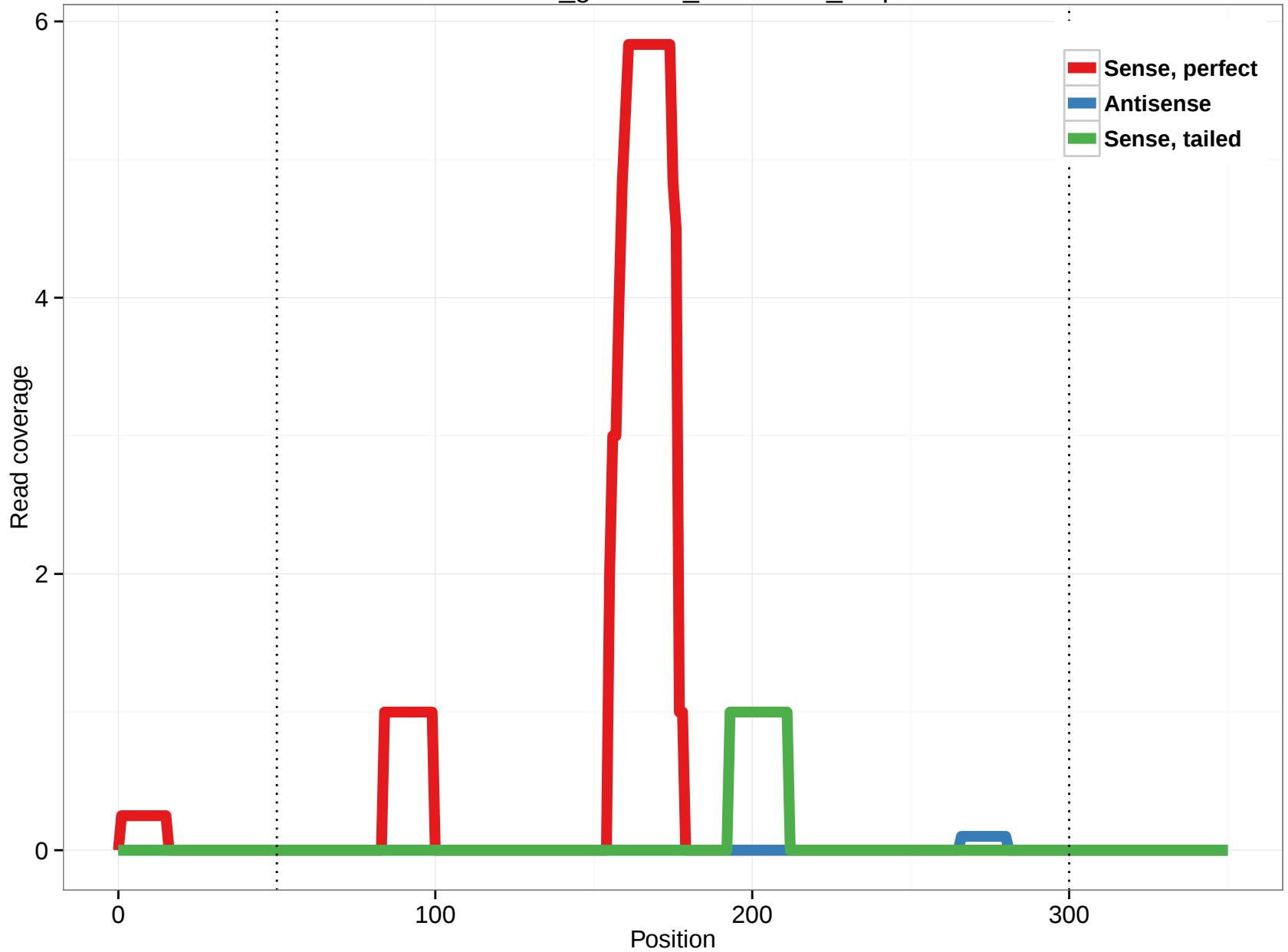
rheMac3_genscan_chr1.2488_1.3p
