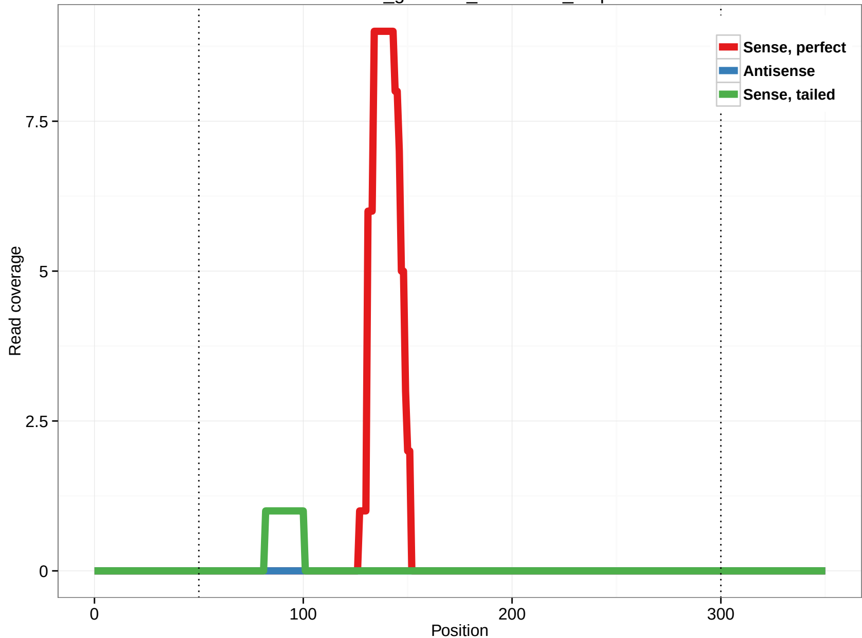
rheMac3_genscan_chr1.2425_3.3p
