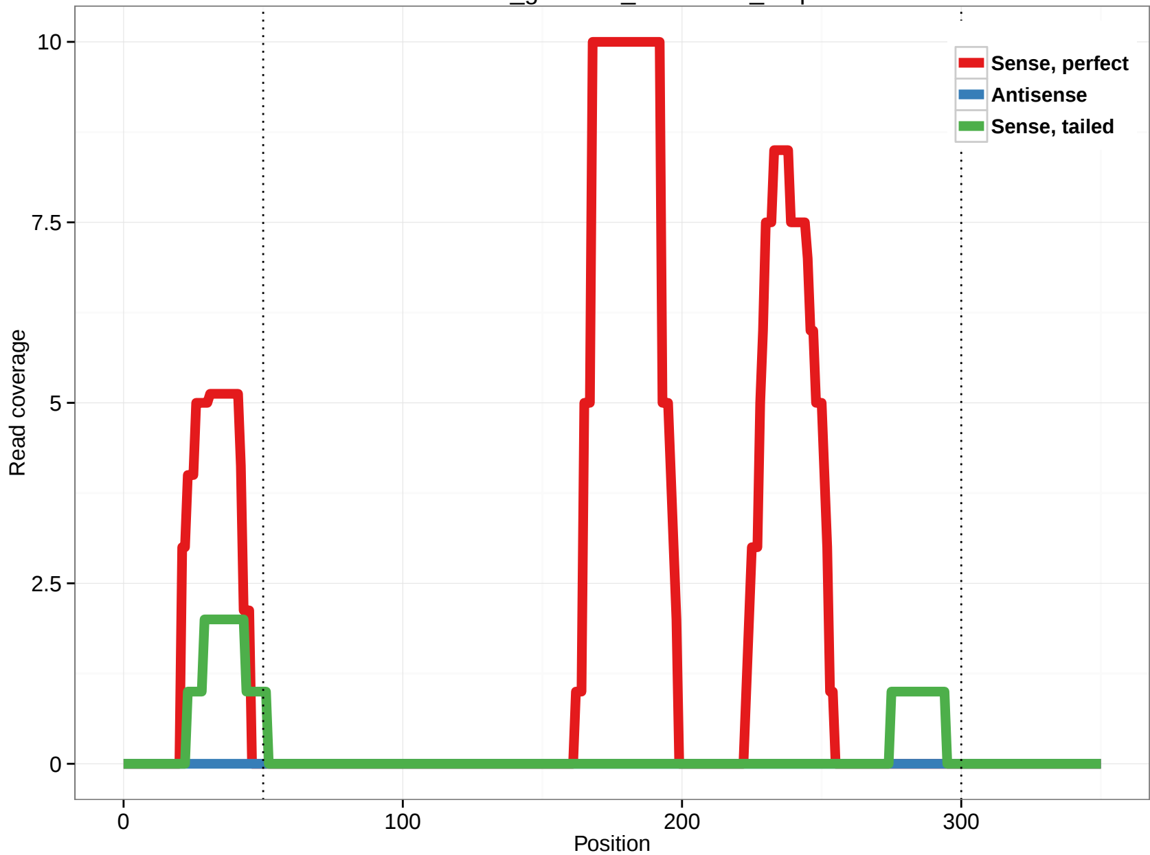
rheMac3_genscan_chr1.2342_9.5p
