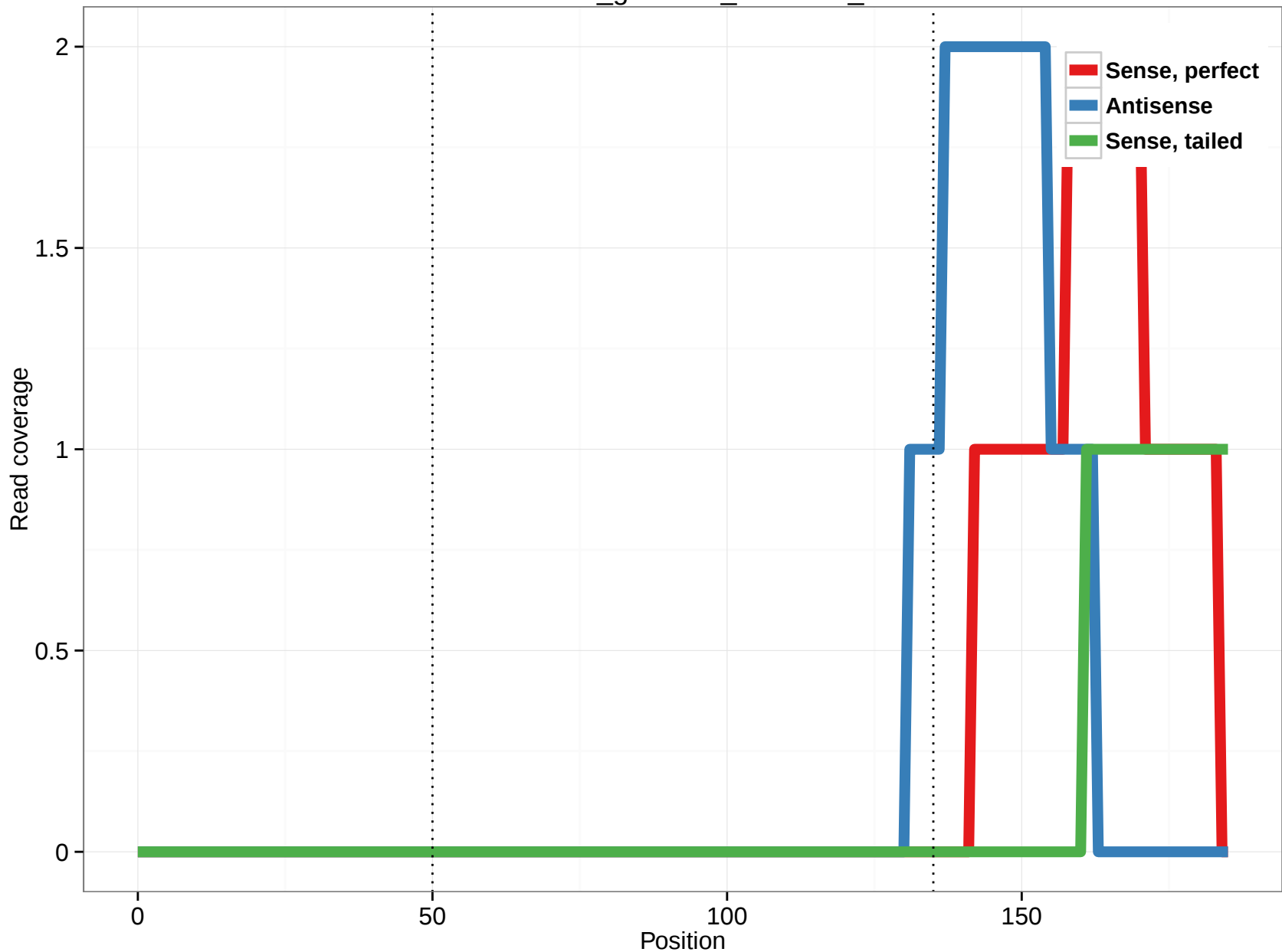
rheMac3_genscan_chr1.232_4
