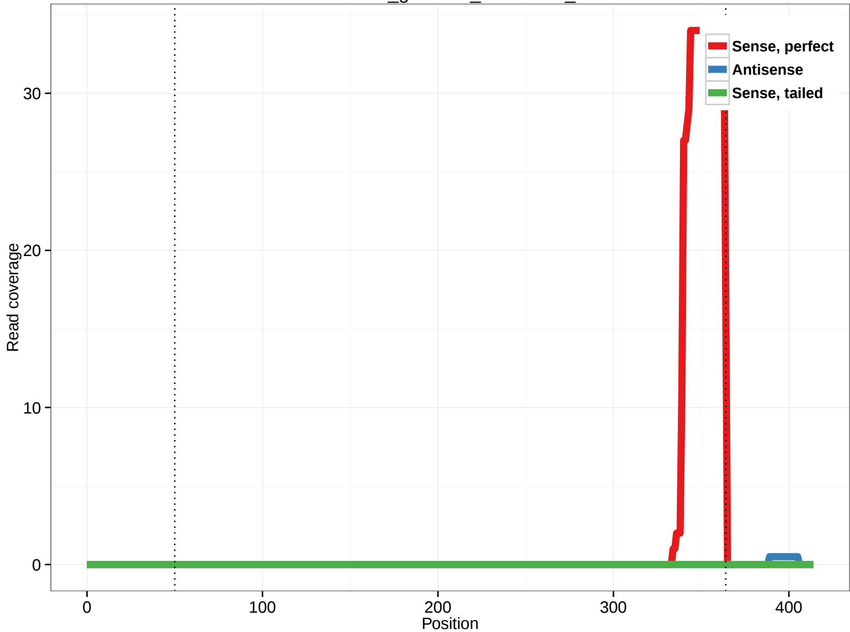
rheMac3_genscan_chr1.2325_2
