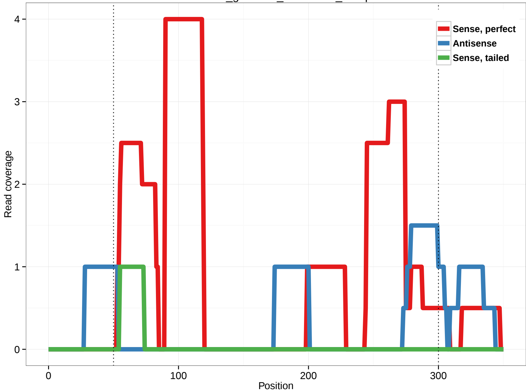
rheMac3_genscan_chr1.2306_19.3p
