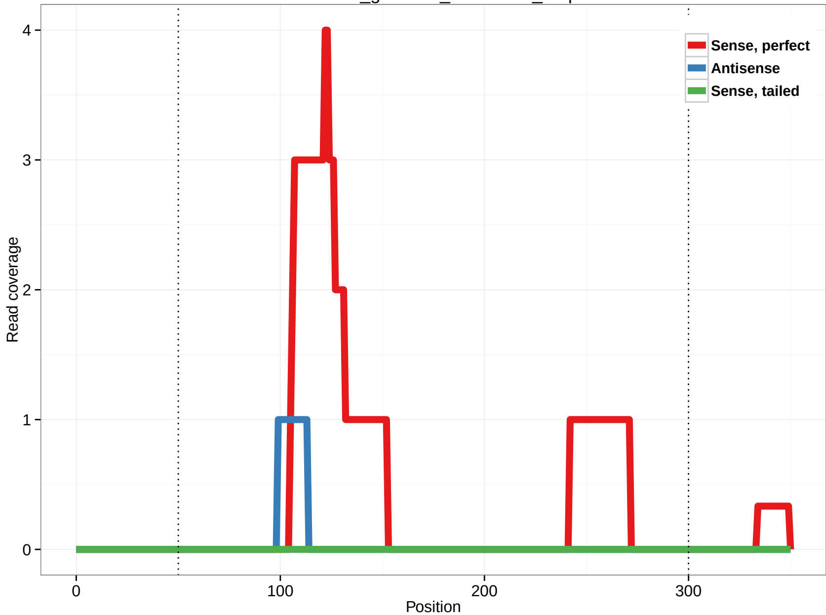
rheMac3_genscan_chr1.2295_7.5p
