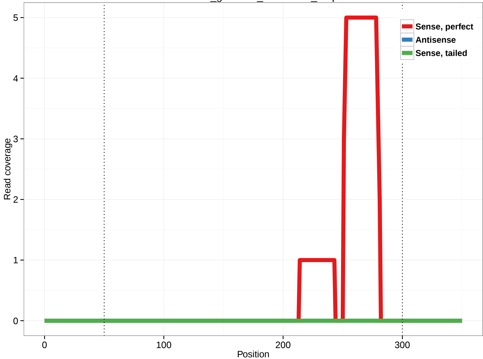
rheMac3_genscan_chr1.2289_5.3p
