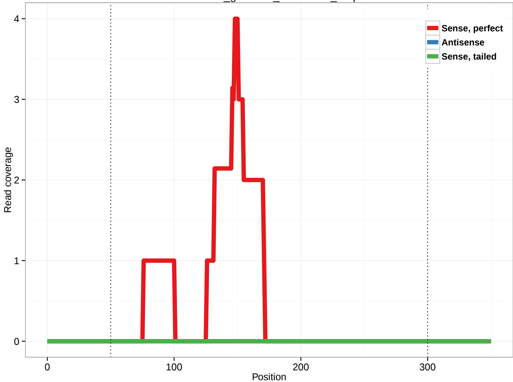
rheMac3_genscan_chr1.2273_2.3p
