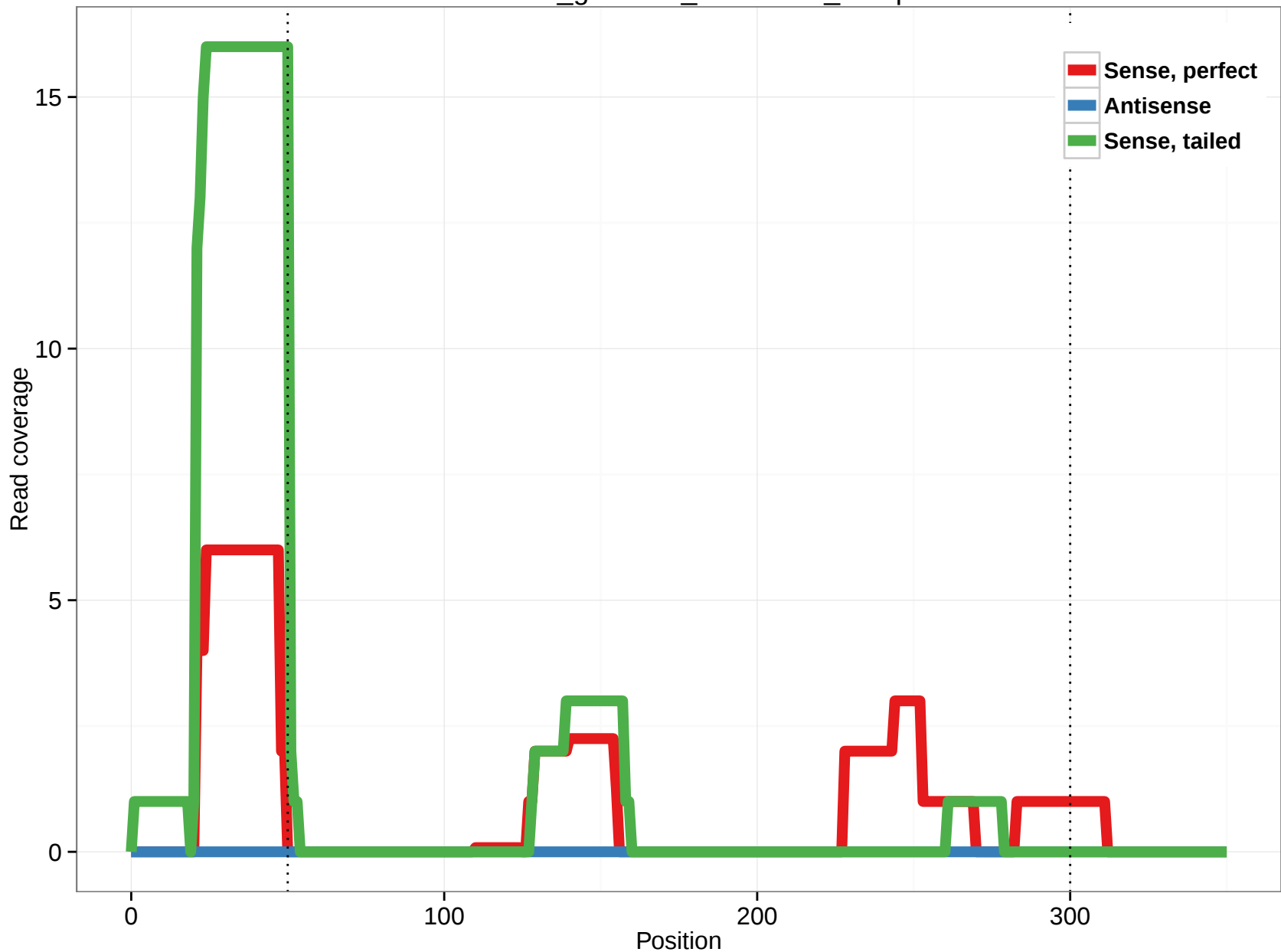
rheMac3_genscan_chr1.2223_24.5p
